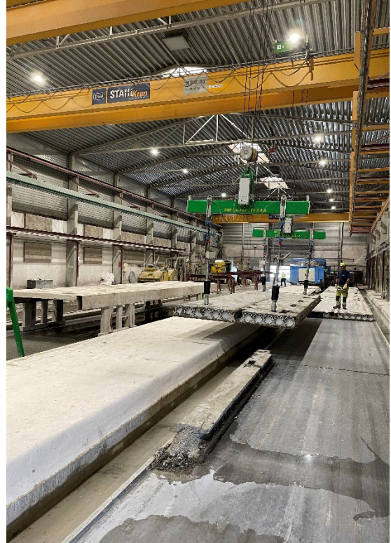
Lifting yoke engaged
